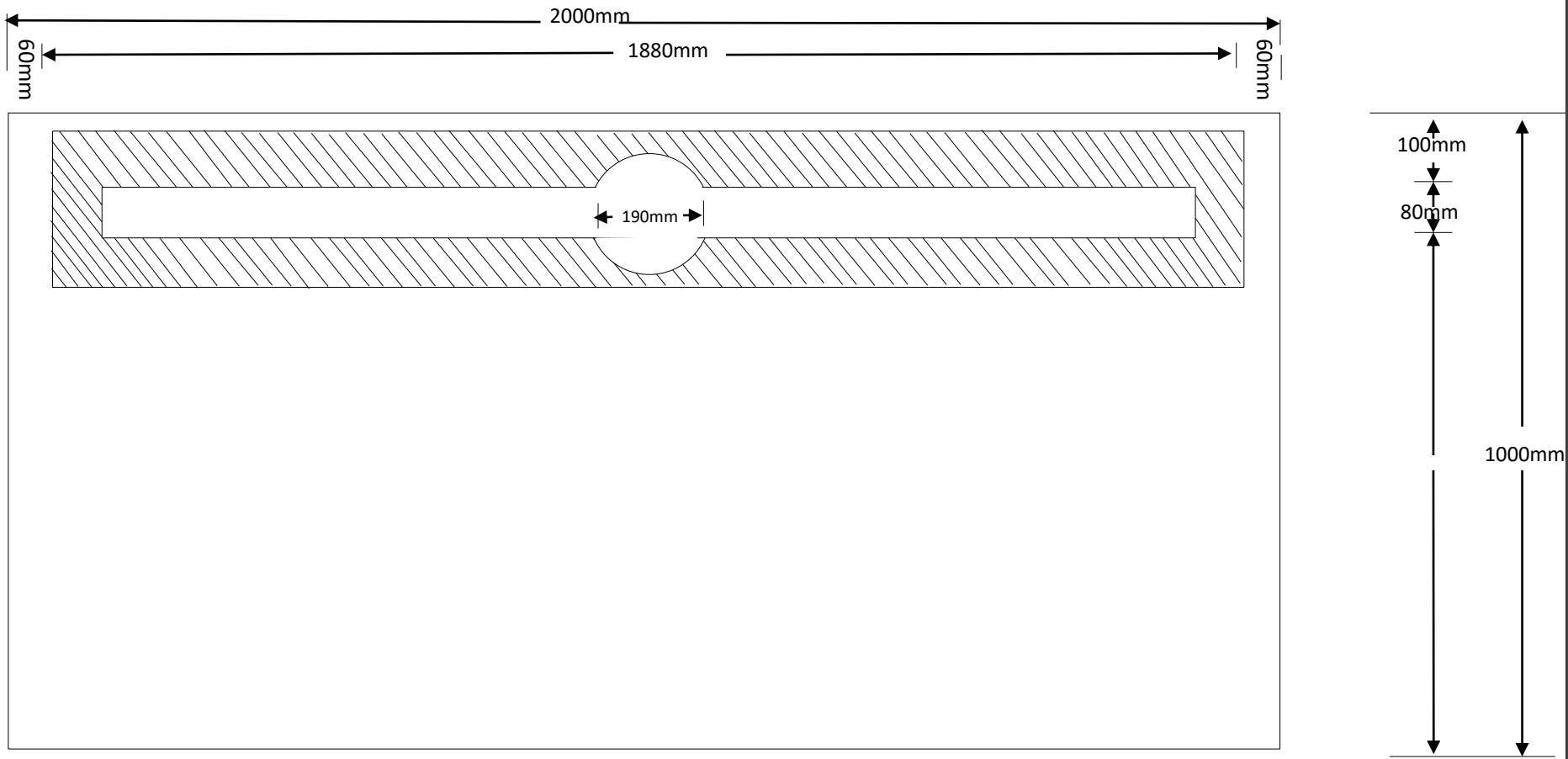
Bottom view
